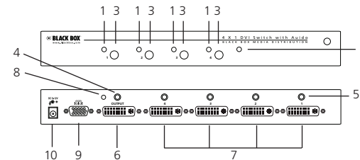
Figure 2-1. 4X1 DVI and Audio switch front and back panels.
